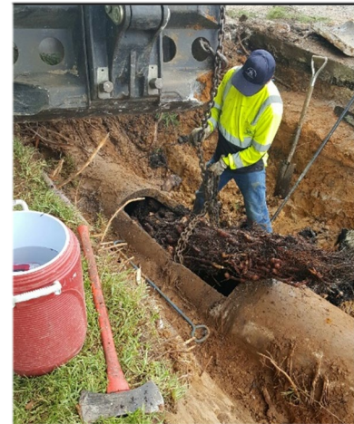
Figure 8 - Removing a Root Wad from a Storm Drain
