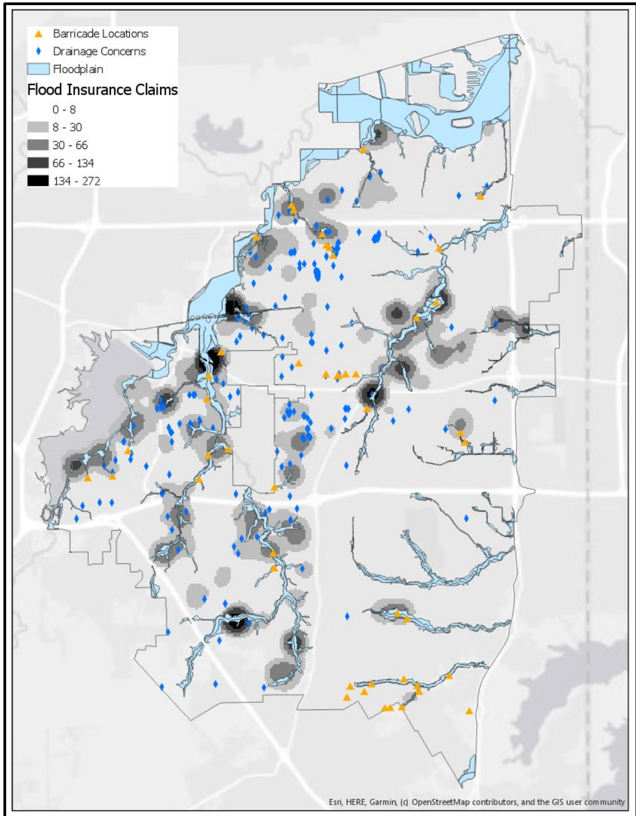
Figure 11 - Citywide Map of Reported Drainage Concerns and Flood Insurance Claims
