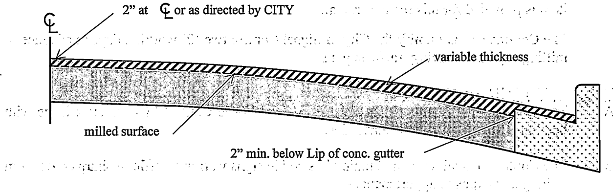
Surface Milling for Full Depth Asphalt Streets with Separate Concrete Curb and Gutter
