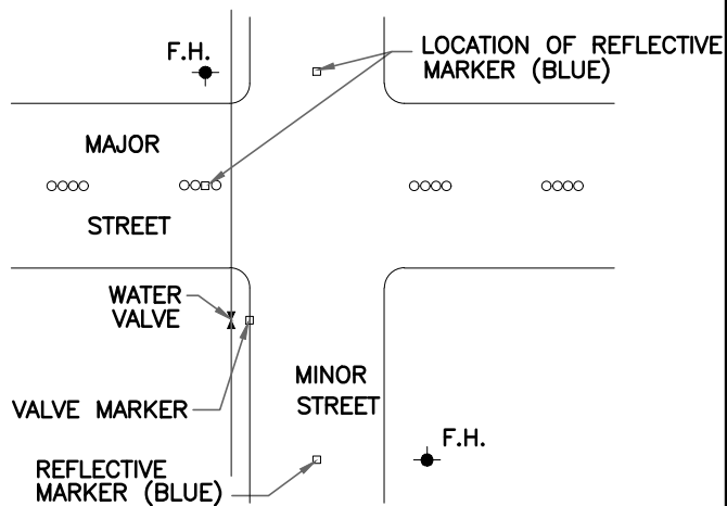
VALVE AND FIRE HYDRANT MARKER LOCATIONS (SEE NOTES THIS DETAIL)
